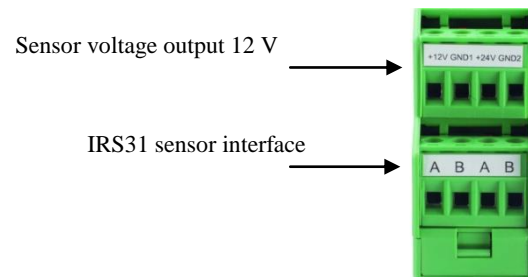
Illustration 1: ISOCON-UMB connection
